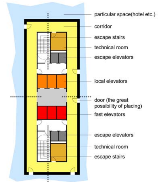
CORE SCHEME 1:500
