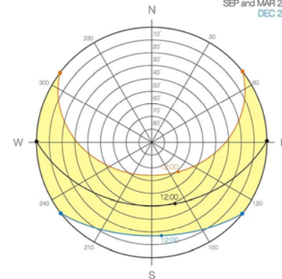
SUN PATH DIAGRAM MANNHEIM, GERMANY
