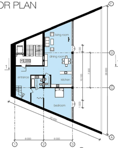
4th FLOOR PLAN
