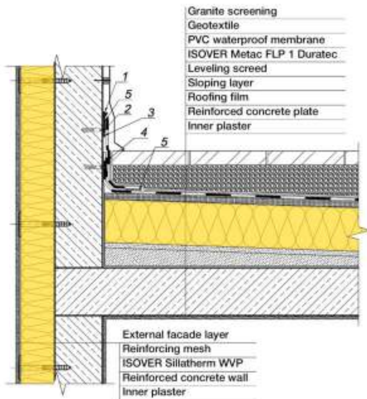
Flat roof detail
