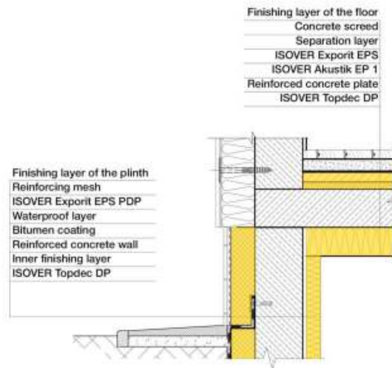
External wall detail
